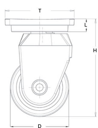
< Side view of caster >
